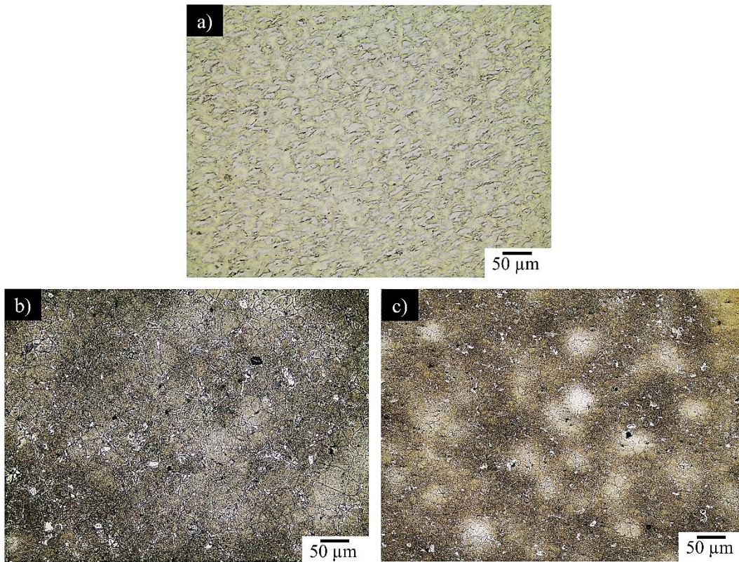
Figure 2. Etched microstructure images of the samples: a) pure Ti, b) Ti-Mn, c) Ti-Mn-Fe
